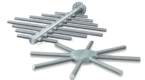
HEADER LATERALS & HUB LATERALS
